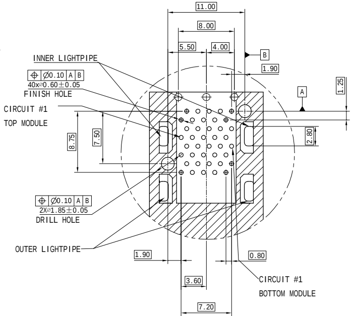
KEEPOUT ZONE DETAIL SCALE 5:1
